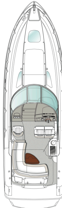
COCKPIT LAYOUT
