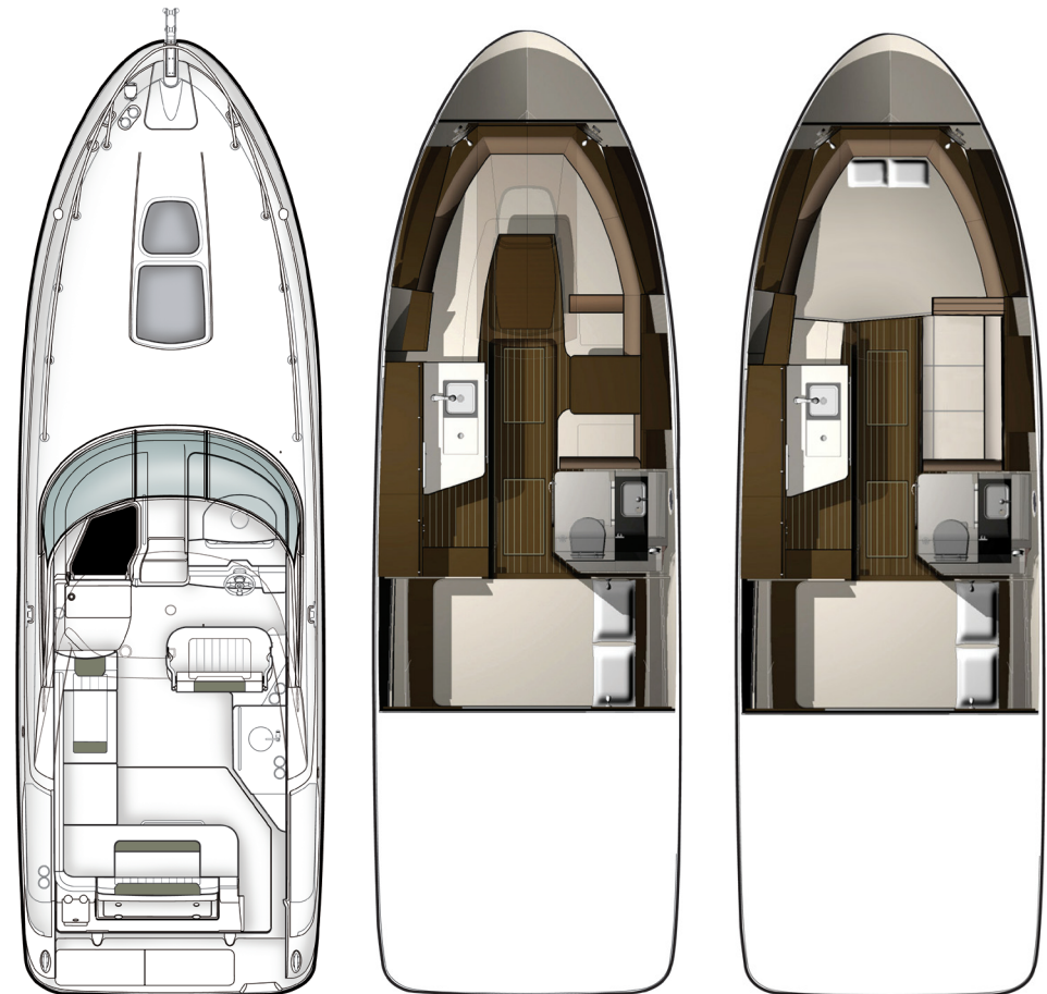
COCKPIT LAYOUT
